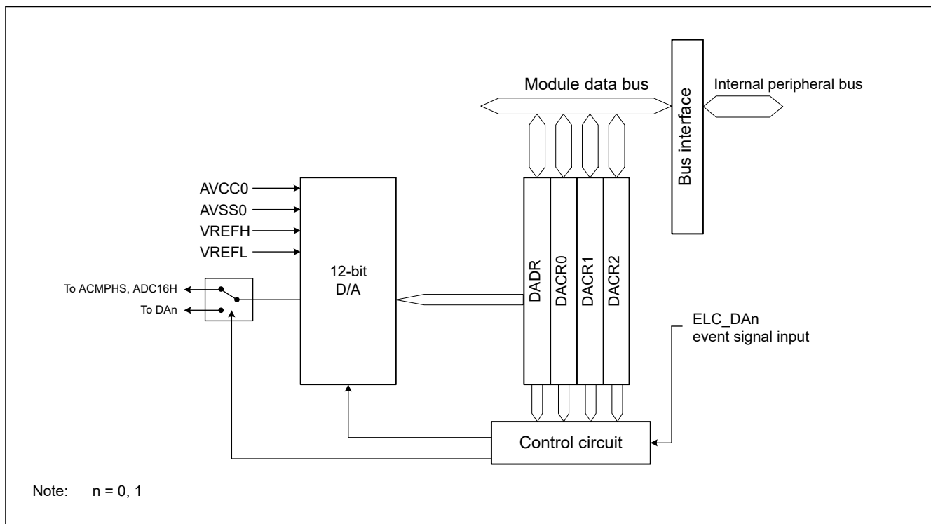
Figure 53.1 DAC12 block diagram
